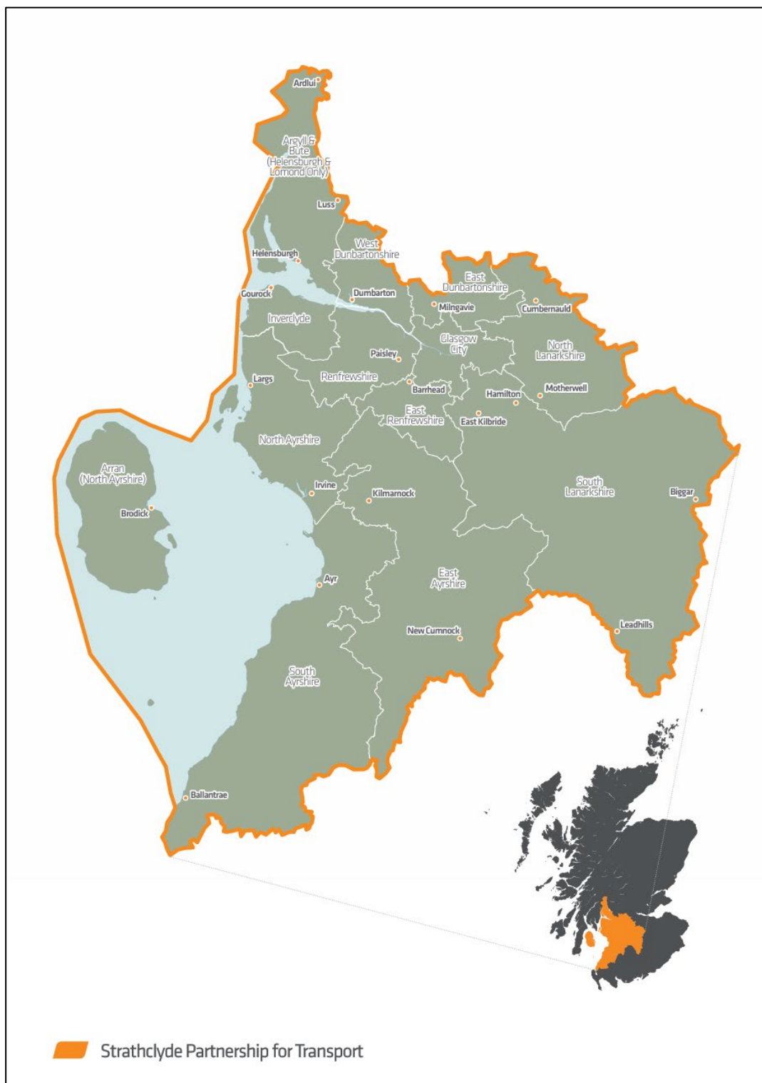
Figure 1.1: SPT Region
